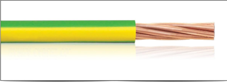
CU/LSOH-XL | 450/750V | BS STANDARD
