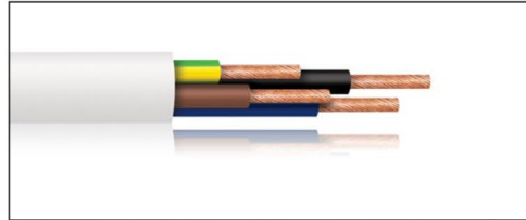
Flexible Cables | 300/500V
