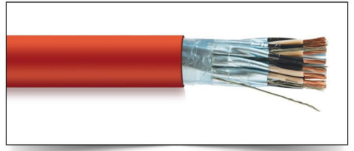
INSTRUMENTATION CABLE FOUNDATION™ FIELDBUS IEC 61158-2 TYPE A, 300V
